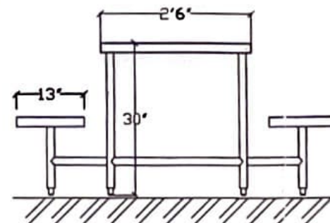
SECTION B-B (WITHOUT FOLDING)
