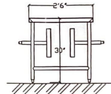
SECTION B-B (WITH FOLDING)
